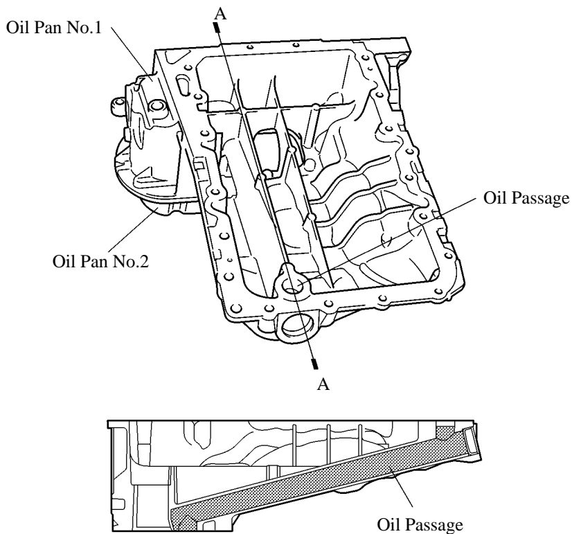
A – A Cross Section
