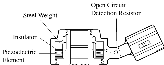
Flat Type Knock Sensor (Non-Resonant Type)
