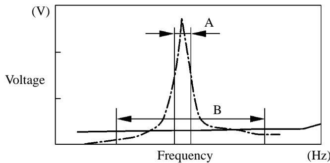
Characteristic of Knock Sensor
