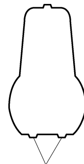
Double-Bead Cylinder Head Cover Gasket Cross Section
